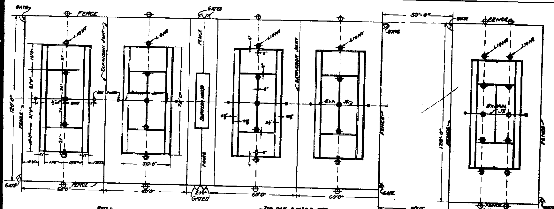
ALL DIMENSIONS ARE OUTSIDE PLAN DETAIL OF COURTS SCALE 1" = 80'
